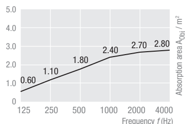
TOPIQ® Sonic element square 1200 x 1200 mm, Suspension height 300 mm
