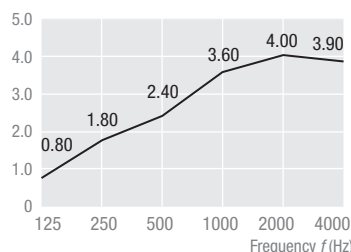
TOPIQ® Sonic element rectangular 1800 x 1200 mm, Suspension height 300 mm
