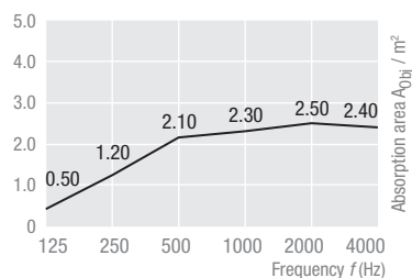
TOPIQ® Sonic element square 1200 x 1200 mm, Suspension height 150 mm
