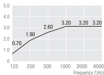
TOPIQ® Sonic element rectangular 1800 x 1200 mm, Suspension height 150 mm
