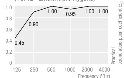
Sound absorption values (TOPIQ® Efficient pro Hygena)
